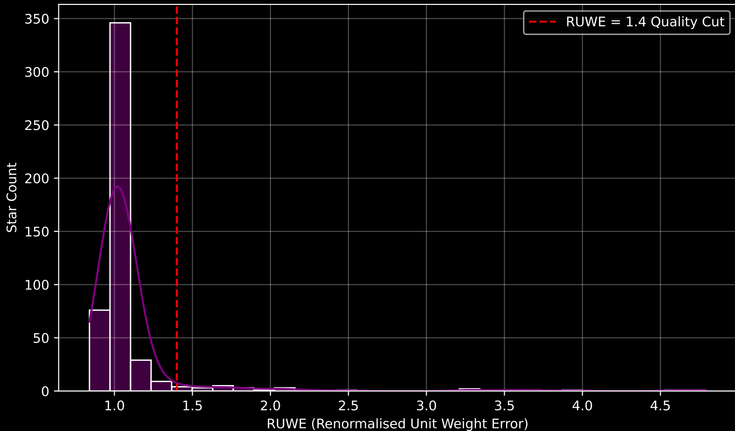
GAPOGEE DR17 Field [090-08] RUWE Distribution (n= 488)
