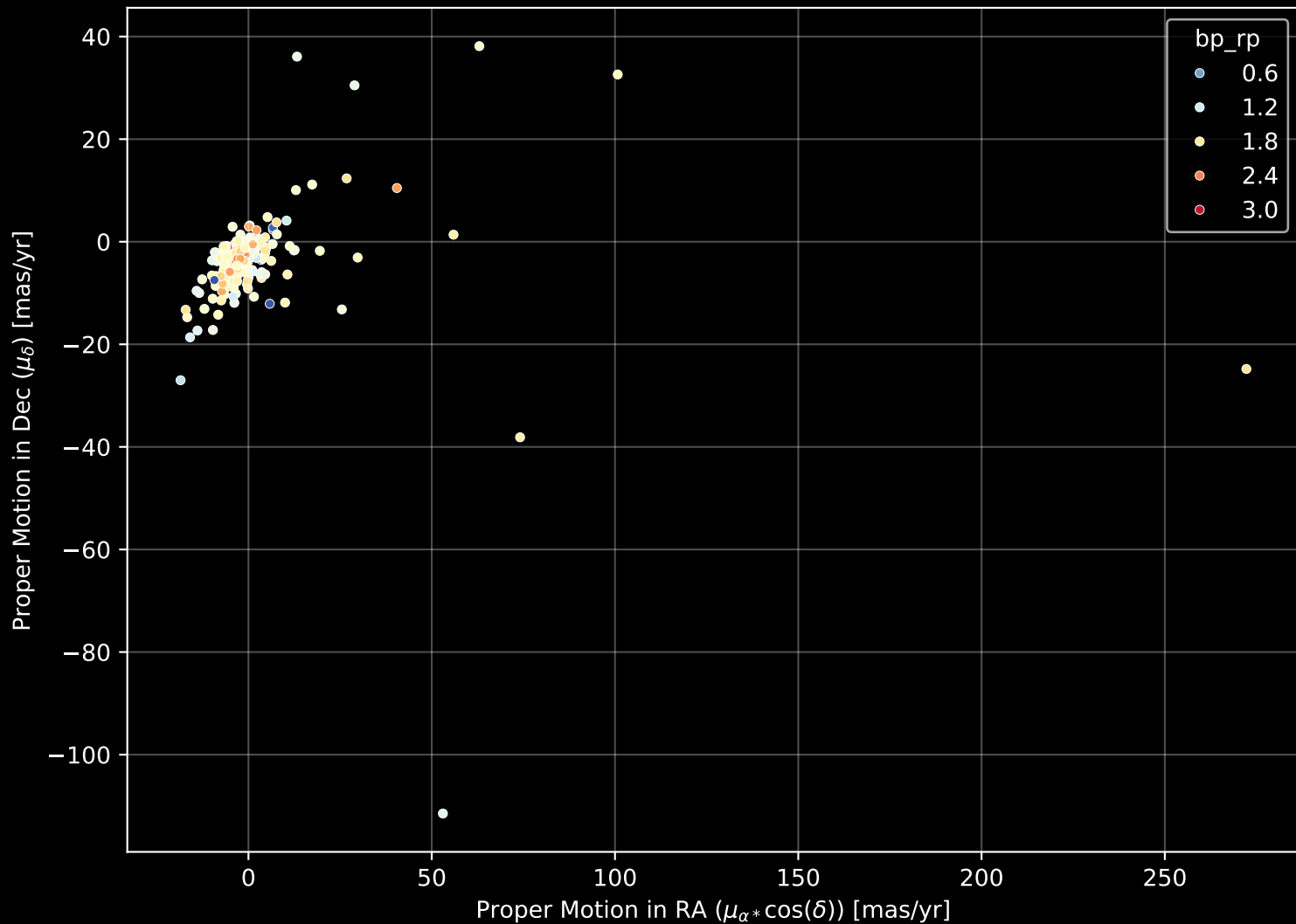
APOGEE DR17 Field: [090-08] Proper Motion Diagram (n= 493)
