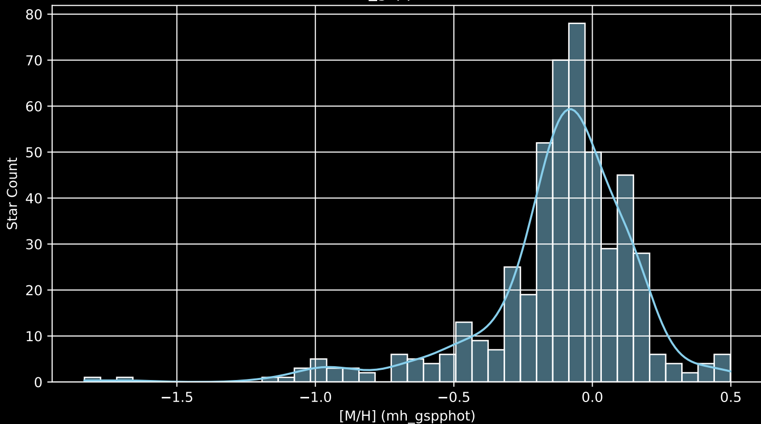
APOGEE DR17 Field: [090-08 [M/H] (mh_gspphot) (n= 488)
