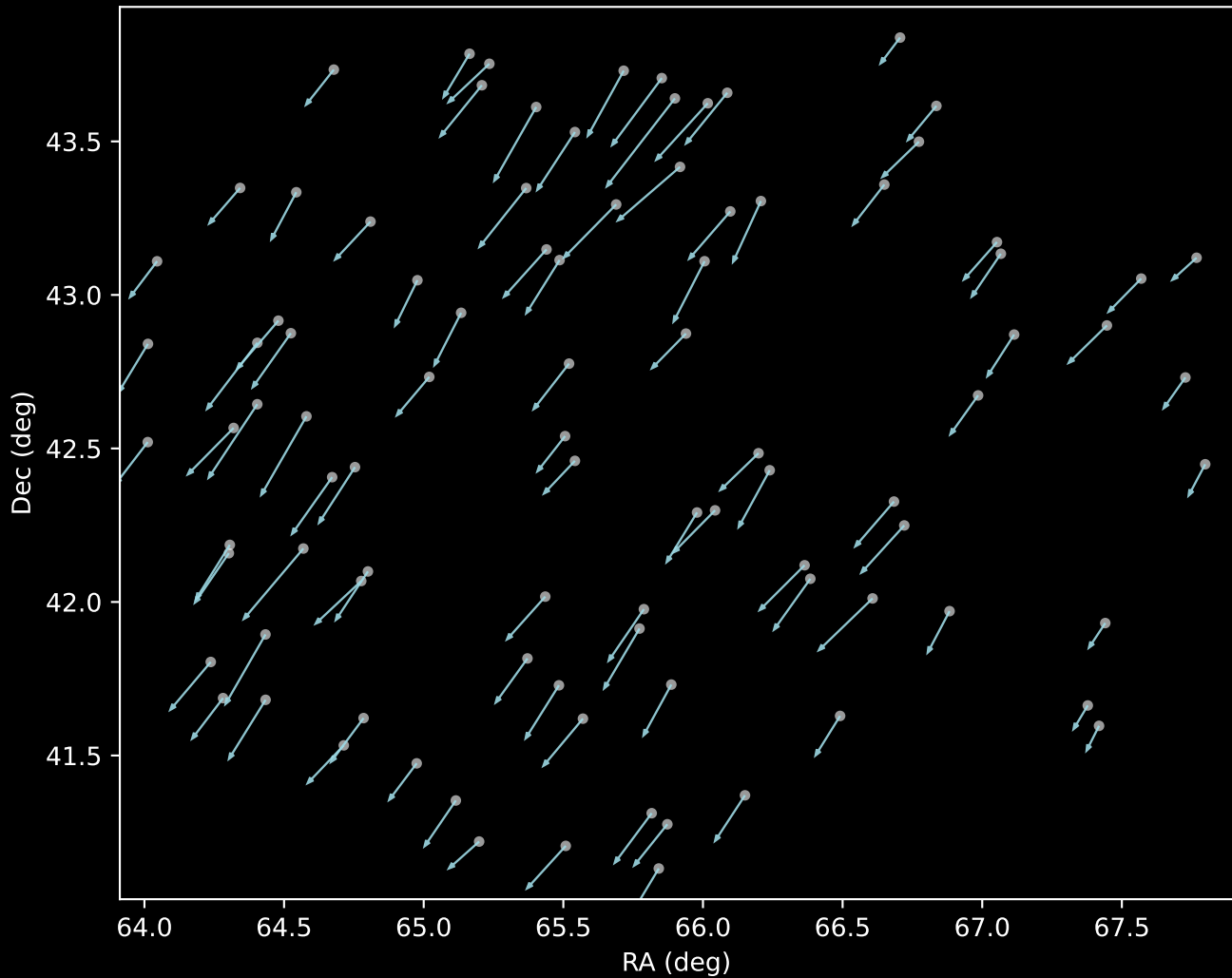
APOGEE DR17 Cluster 19 Proper Motion Vectors (n=93)
