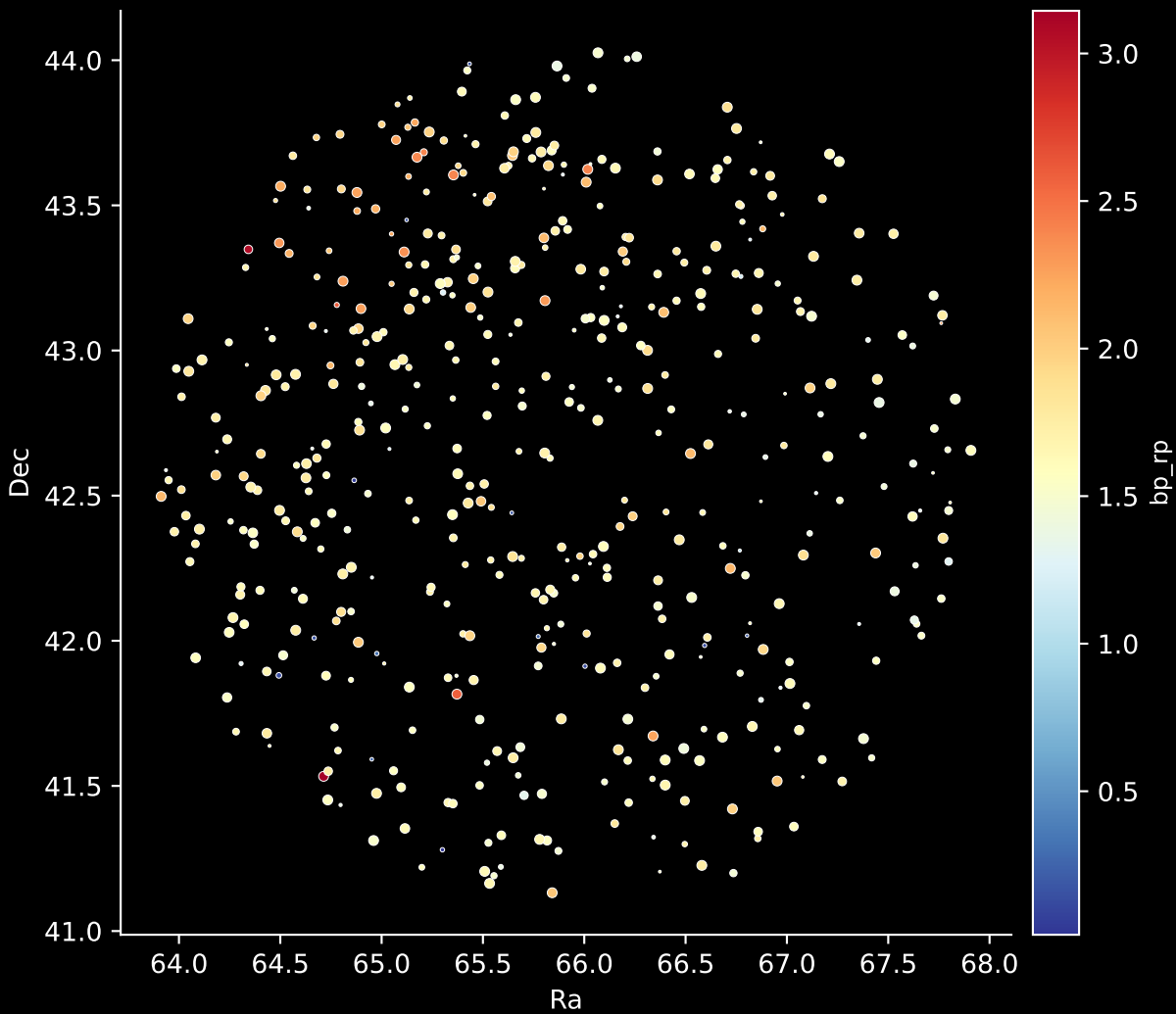
APOGEE DR17 Field: [090-08] Stars: 493
