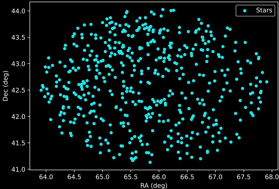
APOGEE DR17 Field: [090-08] Proper Motion Vectors for Gaia Star Field (n= 493)
