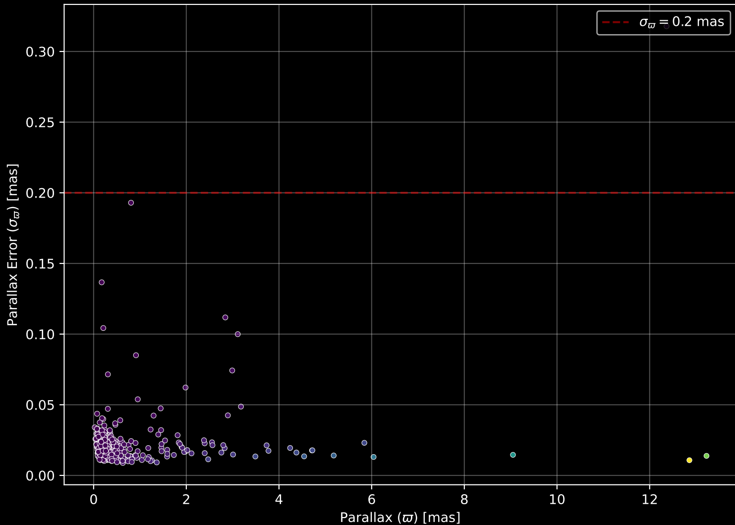
APOGEE DR17 Field: [090-08] Parallax Quality (n= 493)
